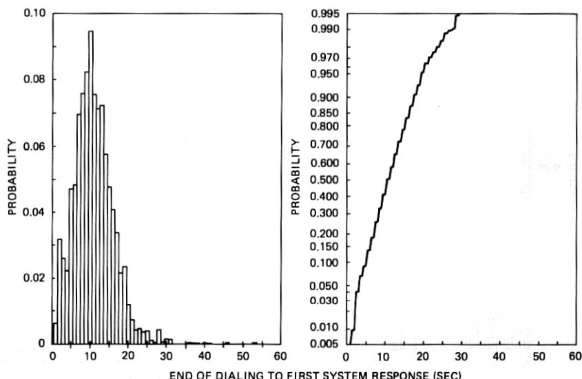
Fig. 5—Distribution of the time from end of dialing to the first system response after dialing a valid telephone number.
